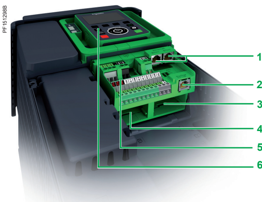
Altivar process drives ports and slots
