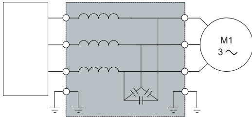
Sinus filter
