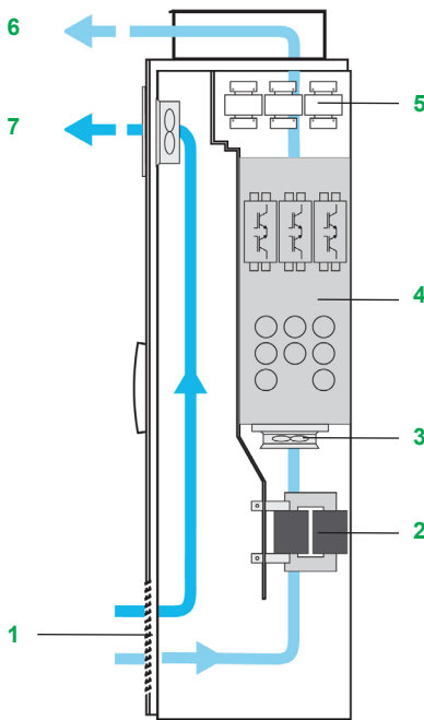
IP23 enclosure
