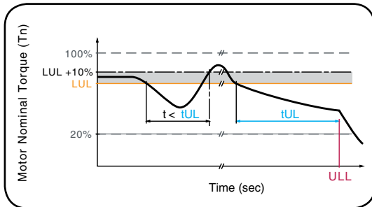
Motor underload detection ( ULL )
