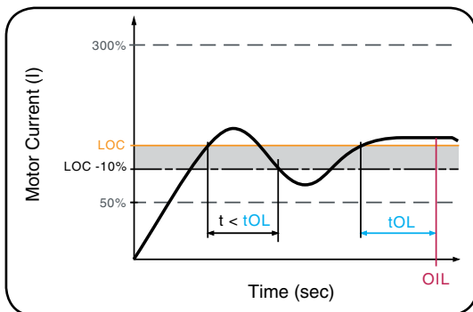
Motor overcurrent detection ( OIL )
