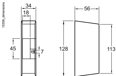
Wall mount accessory
